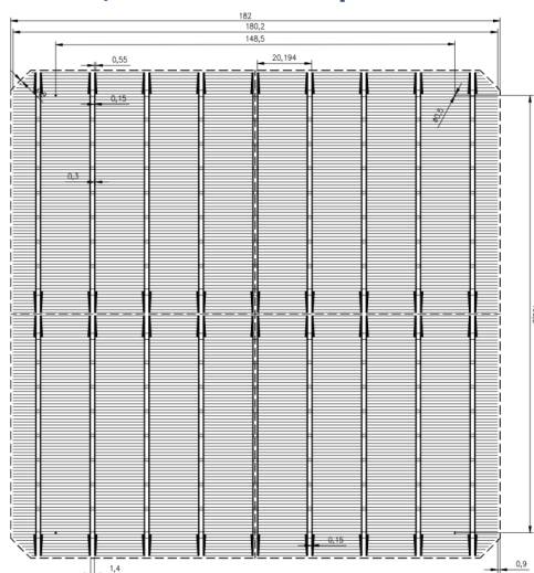
背面电极/Back electrode pattern
